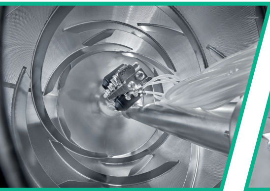
Experience of more than 70 years in mixing were transferred in new baffle design for perfect mixing results.
