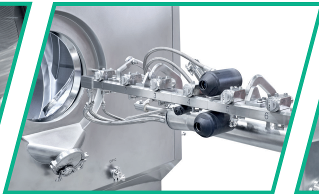
Distance to tablet bed adjustable from outside (manually or fully automatic) without disturbing the coating process.
